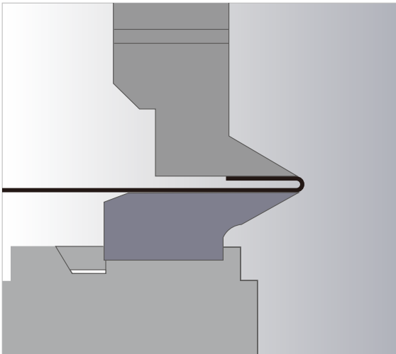
Dead-edge bending
