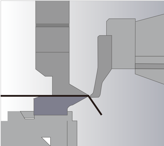
Bend down
