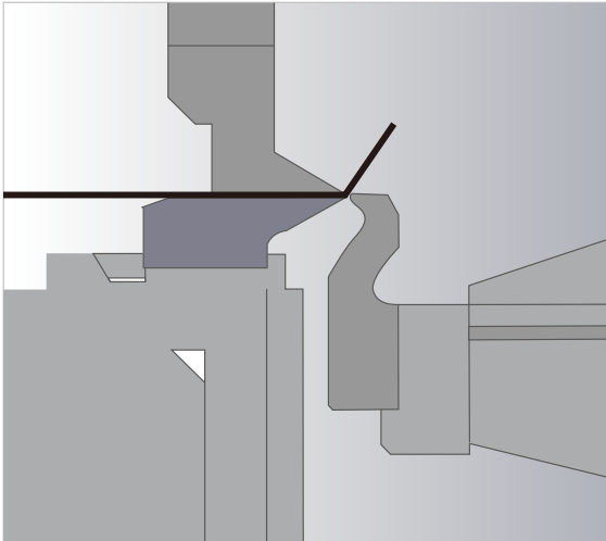
Bend up
